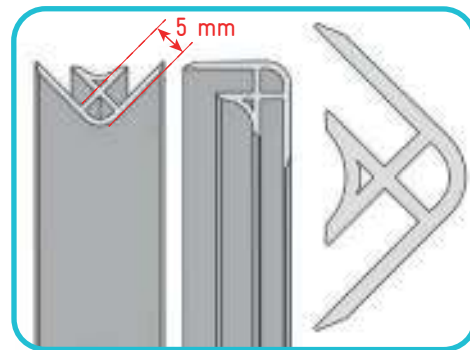
Corner profile
