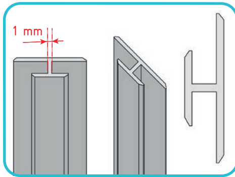
Junction profile
